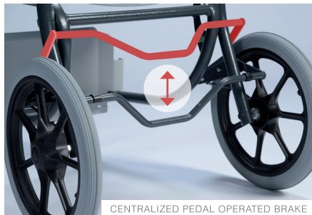
CENTRALIZED PEDAL OPERATED BRAKE
